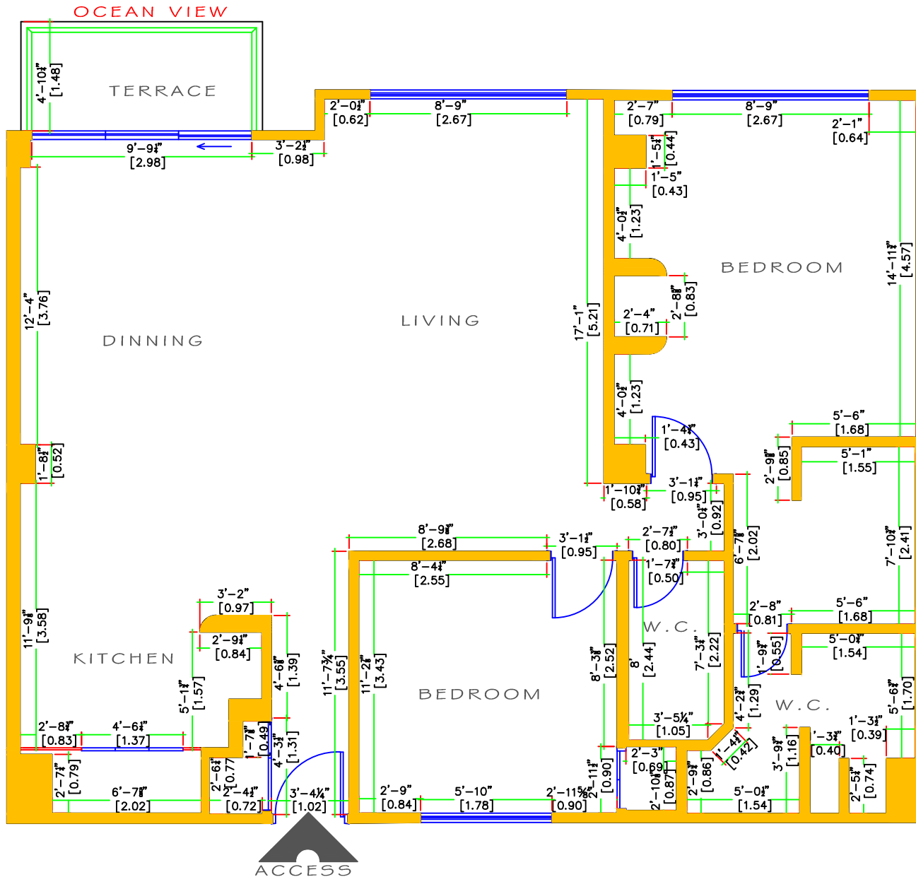
FLOOR PLAN
