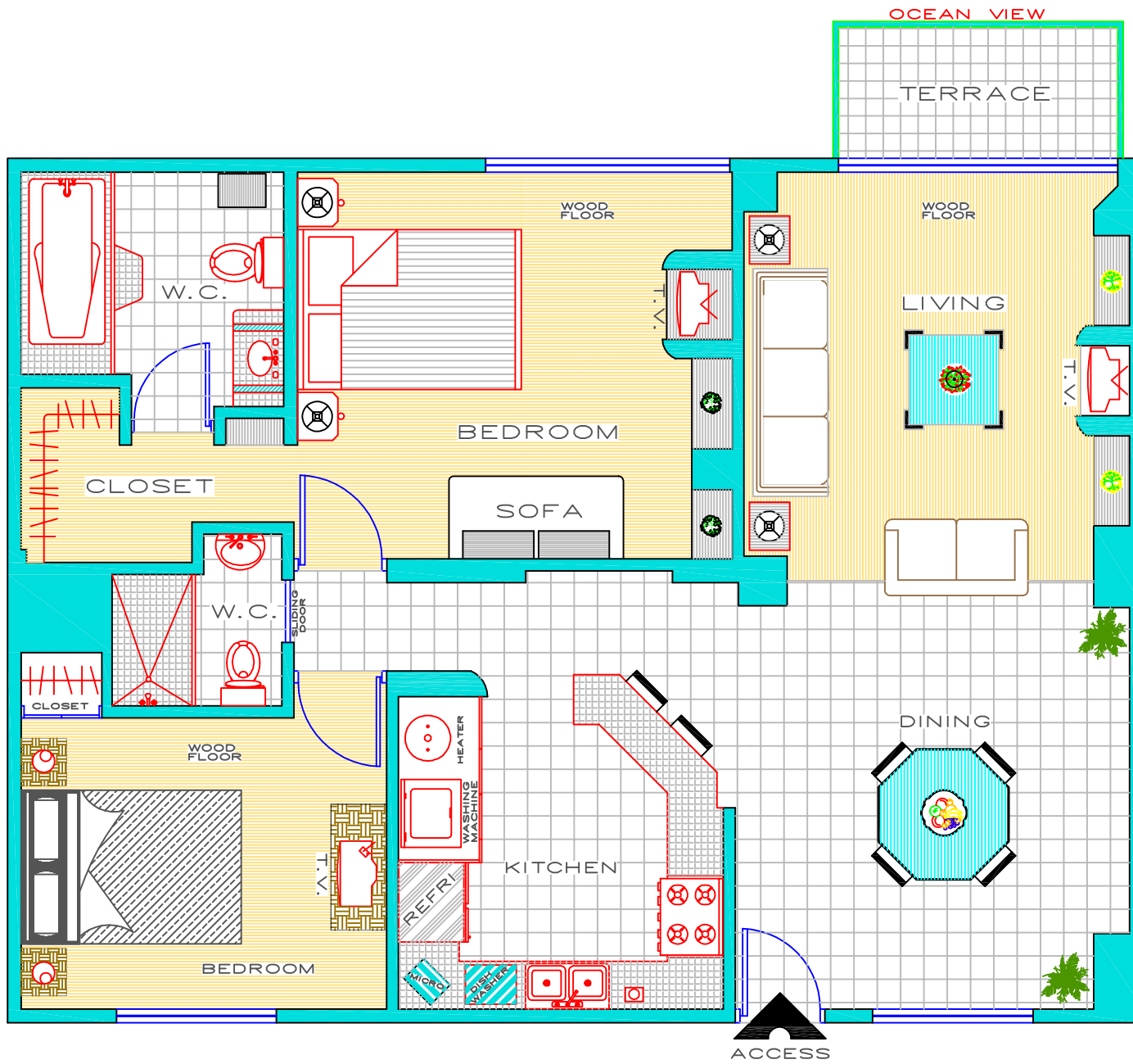
FLOOR PLAN
